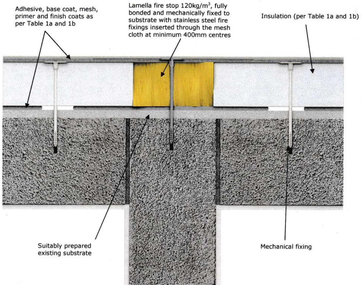
Figure 4: Fire Break Detail
