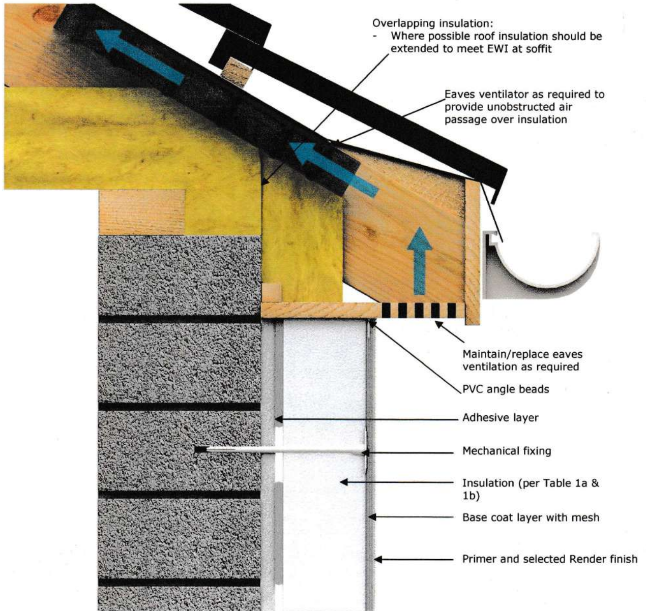
Figure 5: Eaves Detail
